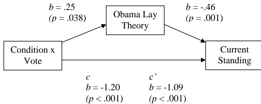
Figure 8. Study 5. Path analysis demonstrating that one's lay theory of President Obama's changeability partially mediates the effect of condition (positive or negative evaluation) by vote (Republican or Democrat) on judgments of how much Obama's performance as Senator should affect his current standing in the national election.
