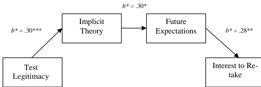
Figure 3. Path analysis using Structural Equation Modeling (bootstrapping, 2000 samples, 95% confidence), Study 2, failure condition. Model fit was excellent. Legitimate failure had a significant and positive indirect effect on expectations of future performance, and a marginal positive indirect effect on interest in re-taking the test. Legitimate failure predicted a more incremental theory of change, which predicted higher expectations of future performance, which predicted increased interest. * p < .05 ; ** p < .01 ; *** p < .001 .
