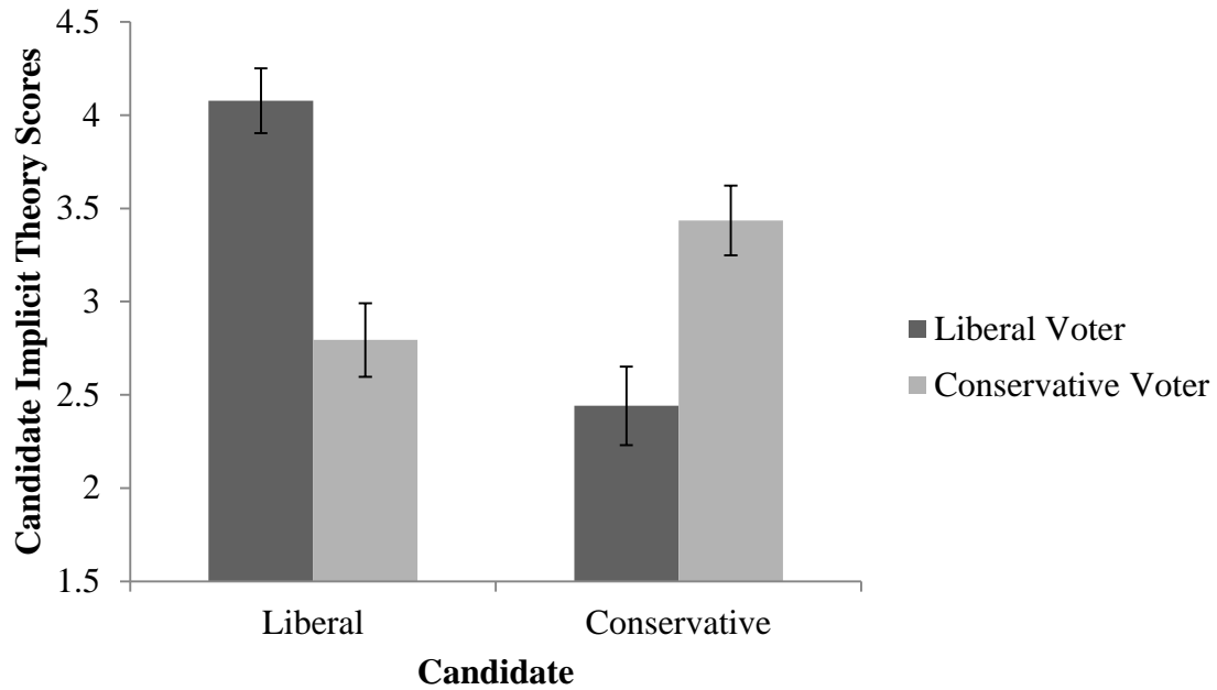
Figure 4. Candidate implicit theory scores as a function of condition and political affiliation (Study 4). Higher numbers indicate more changeability (incremental theory). Means are adjusted for covariates.
